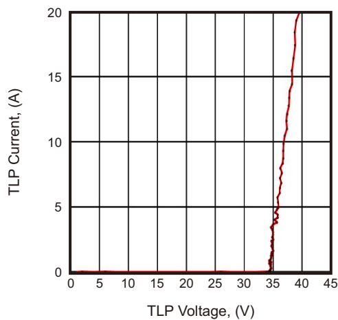
Fig.5 - TLP-Positive Pulse
